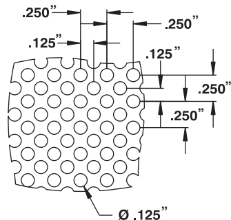
PERFORATION DETAIL
